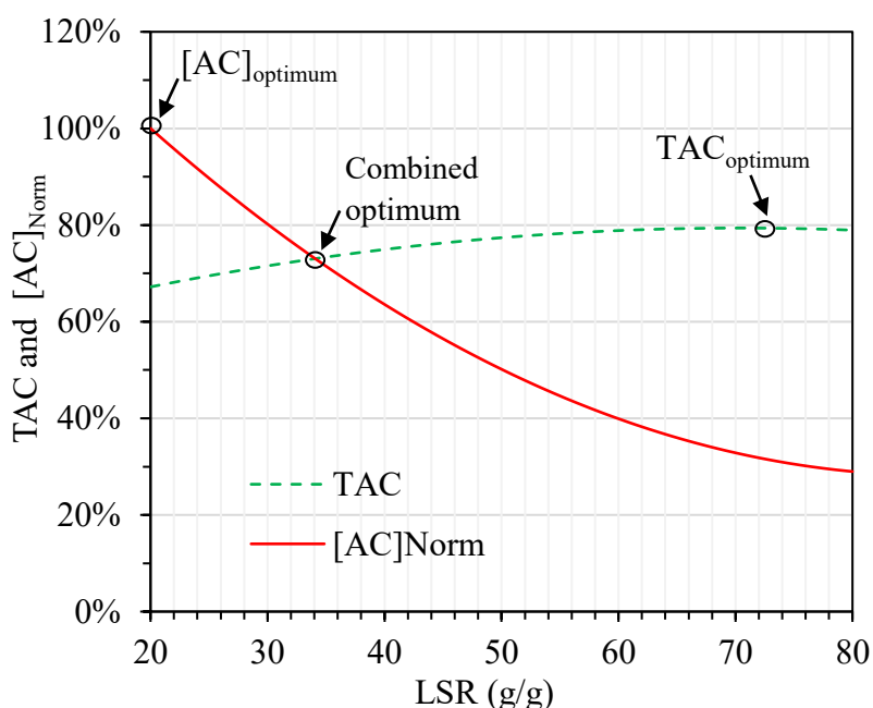
Fig. 5 Variation of the predicted value of TAC and normalized [AC]_{\text{Norm}} for different liquid-solid ratios (LSR). Constant parameters: T: 45 °C; CA: 1.5 % wt.
