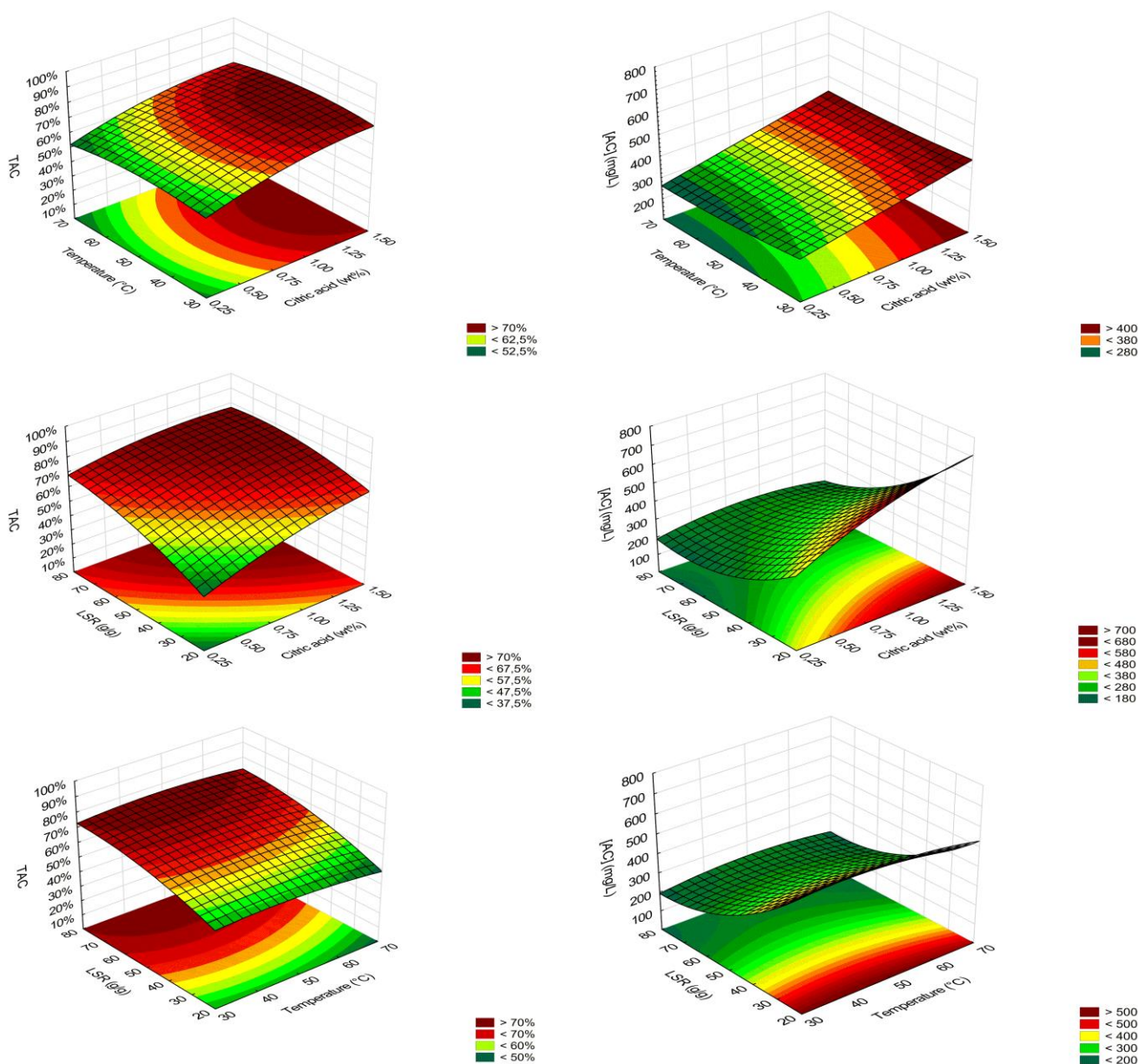
Fig. 4 Response-surface plots showing the effect of the independent factors (T, °C; CA, % wt.; and LSR, g/g) on TAC, % and [AC], mg/L.
