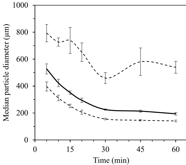
Fig. 1 Median particle size of the suspension during homogenization (full line). The dashed lines illustrate the interval of particle diameters where 80 % of the particles are found. Operating conditions: CA: 0.75%; T: 50°C; LSR 50 g/g.
