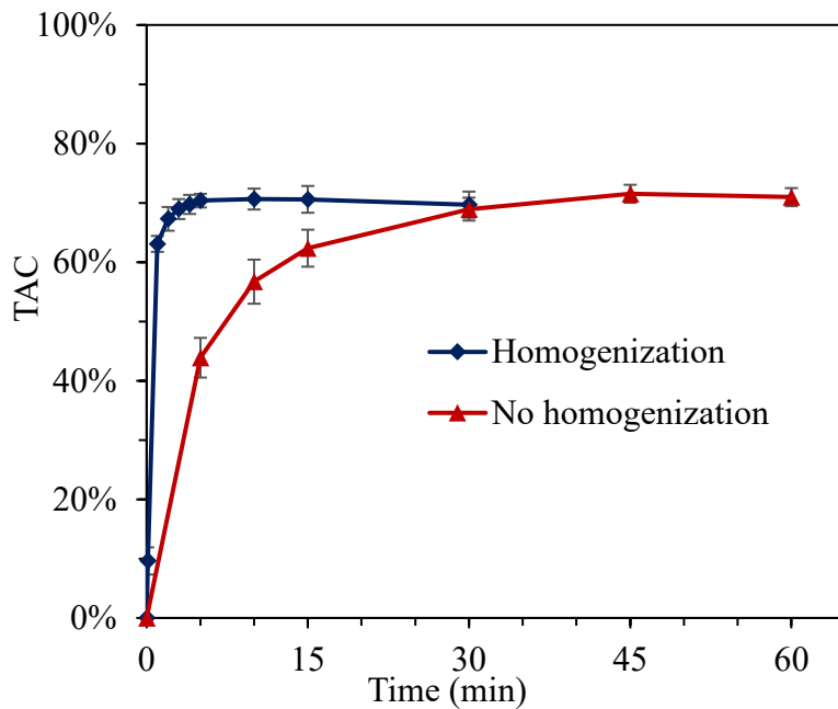
Fig. 2 Total anthocyanin content (TAC) extracted with and without homogenization, with respect to time. Operating conditions: CA: 0.75%; T: 50°C; LSR 50 g/g.
