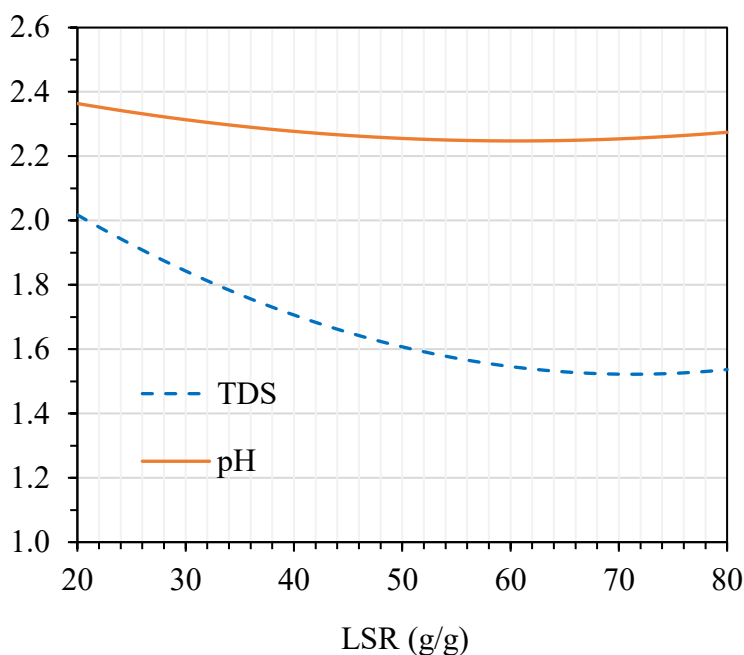
Fig. 6 Variation of the predicted value for total dissolved solids (TDS) and the pH of the extract for different liquid-solid ratios (LSR). Constant parameters: T: 45 °C; CA: 1.5 % wt.
