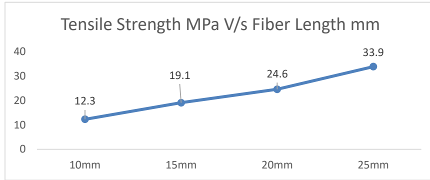
Figure 4. Tensile strength vs Fiber length
