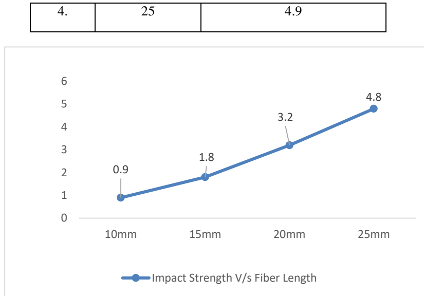
Figure 6. Graph between Impact strength and fiber length.
