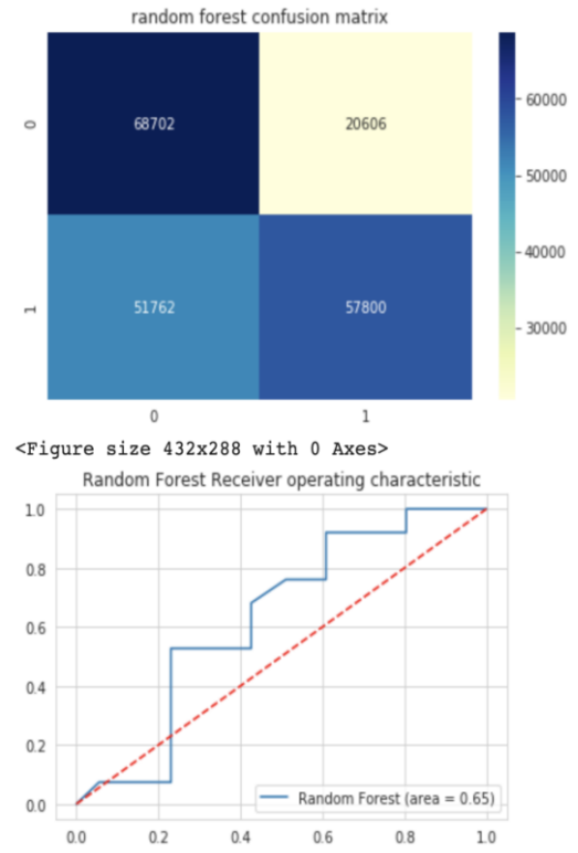
Figure 9. Metrics table, feature importance, confusion matrix and ROC curve of RF.
