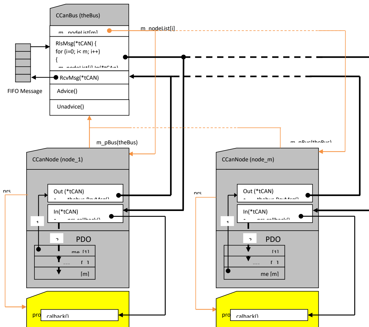
Fig.2: Interaction diagram of the objects in Can Bus Simulation Model, CBSM.
