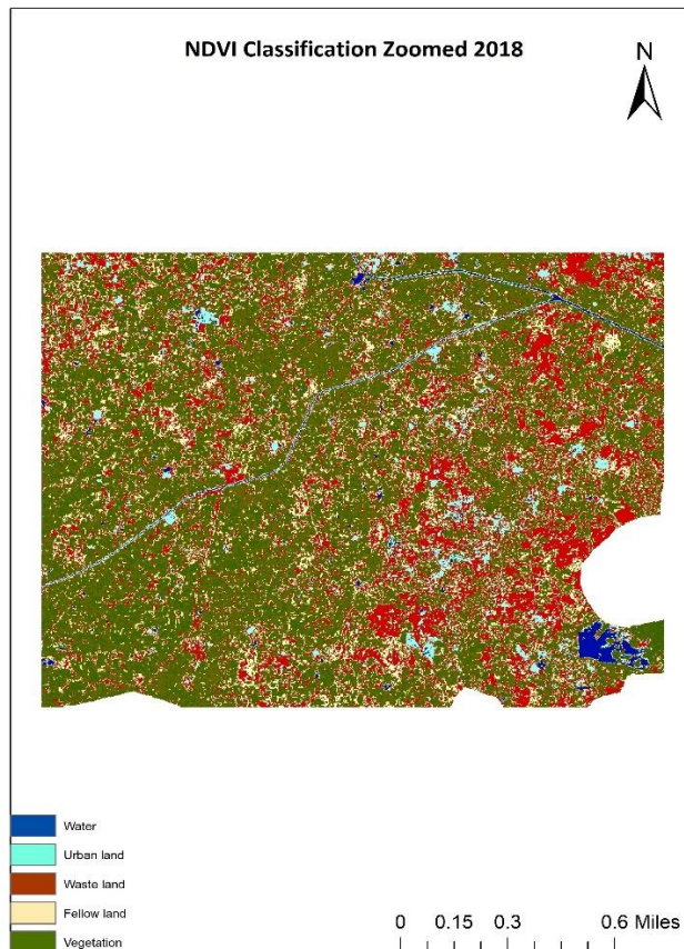
Figure 5: NDVI and FCC of year 2018
