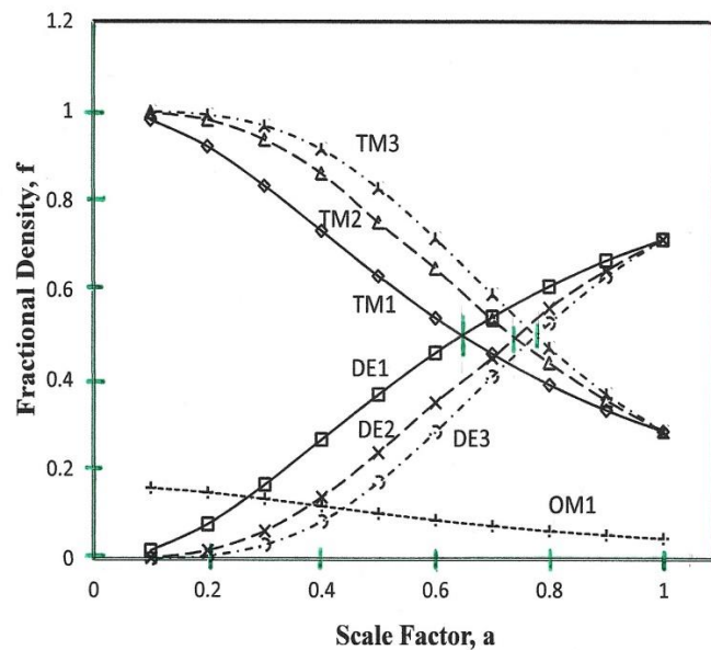
Fig.3- Fractional Energy Density (f) vs Scale Factor (a) DE1- Dark Energy,; DM1-Dark Matter; OM1-Ordinary Matter; TM1- Total Matter for w_s = - 0.7 ; DE2, TM2 for fit with cosmological constant, w = -1 ; TM3, DE3-for fit with Phantom Energy model, w = -1.2
