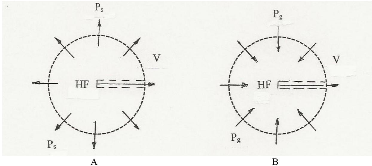
Fig 5. Schematic of the Universe during the period of deceleration (A) and acceleration (B)
