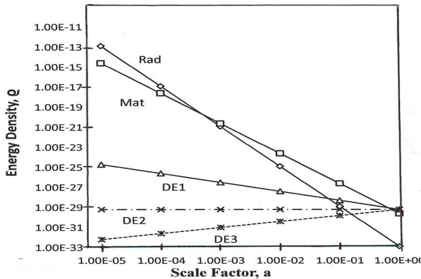
Fig 4. Energy Densities ( \rho , g/cm^3 ) vs Scale Factor ( a ) for 3 models of Dark Energy; Rad-total radiation; Mat-total matter; DE1-Dark Energy with w_s=-0.7 ; DE2- w = -1.0 (Cosmological Constant); DE3- w = -1.2 (Phantom Energy Model)
